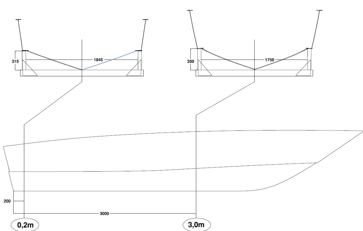
Image: Storage cradle dimensions.
