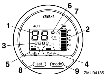
1. Tachometer 2. Trim meter 3. Hour meter 4. Low oil pressure warning indicator 5. Overheat warning indicator 6. Water separator warning indicator 7. Engine trouble warning indicator 8. Set button 9. Mode button
